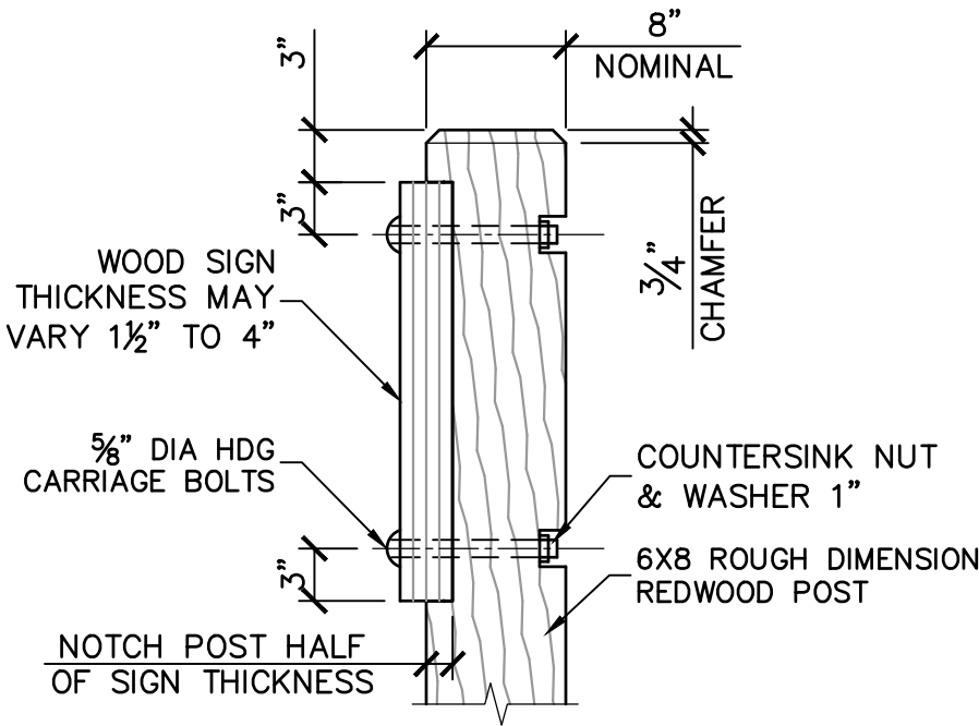
(A) SECTION A-A
