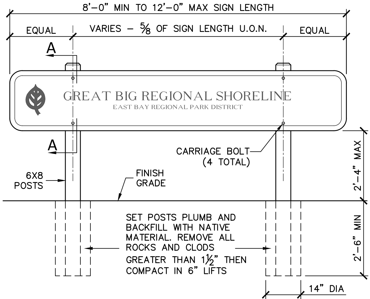
(B) FRONT ELEVATION
