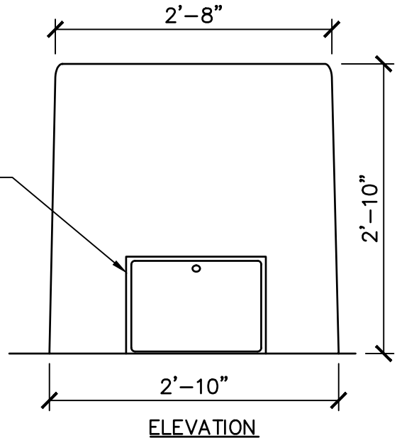
(A) HOT COAL RECEPTACLE - PLAN AND ELEVATIONS
